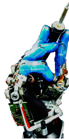
Figure 1: The DLR Hand II executing a pinch grasp on a solder pen
