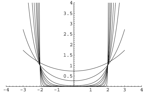
Figure 10: Plot of terms for modeling bound constraints ( p_k^b \in \{0.25, 0.5, \dots, 20\} , \Theta^{\text{low}} = -2 , \Theta^{\text{up}} = 2 )
