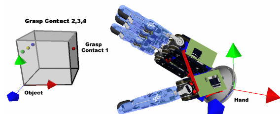
Figure 2: How to find a hand configuration (wrist frame, finger joints) for a given grasp contact set?
