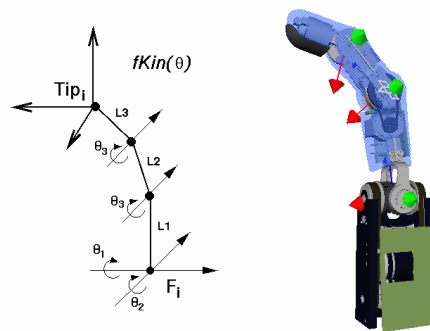
Figure 4: DLR Hand II kinematic model of finger.
