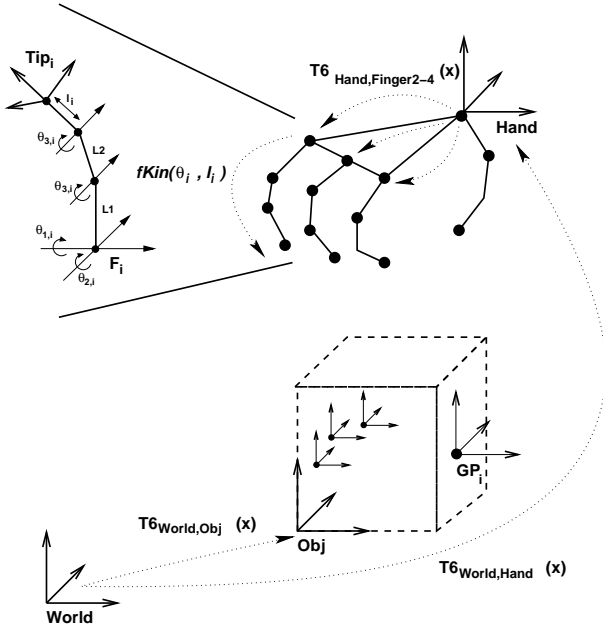
Figure 8: Kinematic description of a hand grasping an object
