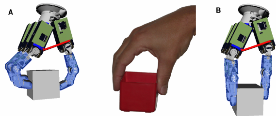
Figure 5: Typical robot (A) and human (B) precision grasp shape
