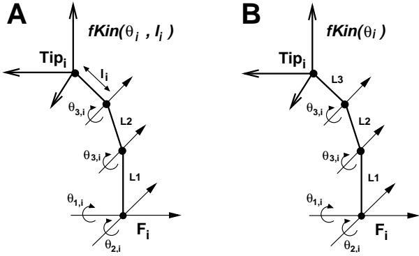
Figure 7: Finger kinematics with (A) and without virtual prismatic joint (B)
