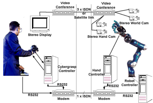
Fig. 5. Telematipulation setup with hand and arm
