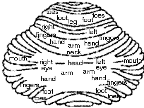
Figure 3. Microzones in the cerebellum.
